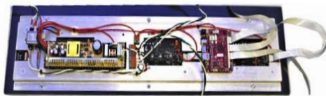
Master Insert with waterproof cover removed
